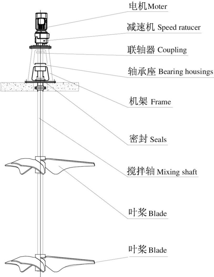
外形安装图 Diagram of the outside dimensions
