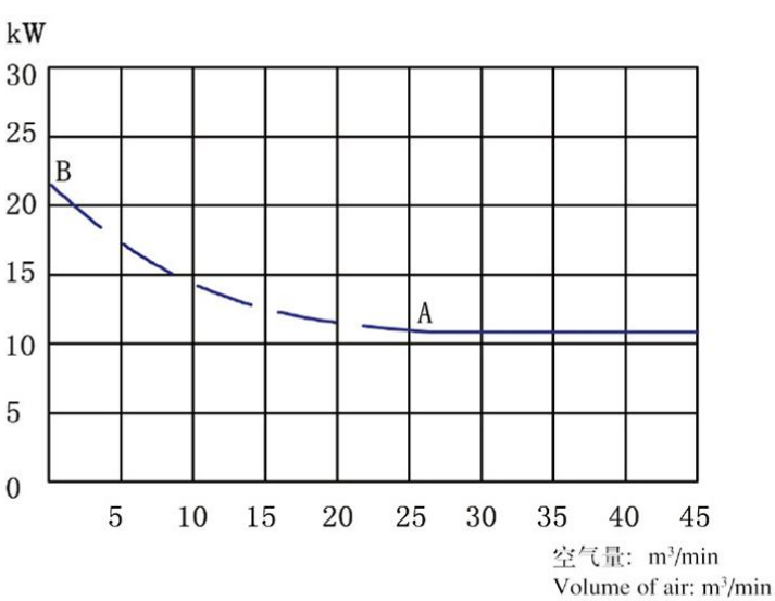
QSB22功率消耗曲线 Curve of power consumption for QSB22
