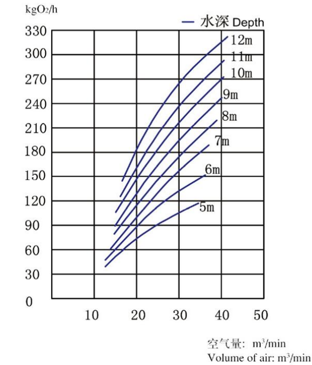
QSB22溶氧性能曲线 Curve of oxygen-dissolving performance for QSB22
